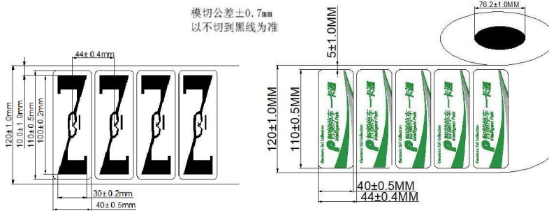
Un-winding Direction/Label Facing Outside 出卷方向图
